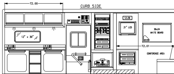
FLOORPLAN "B"
