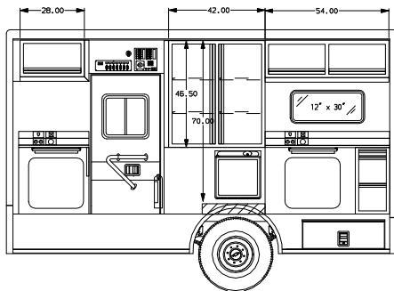
FLOORPLAN "A"
