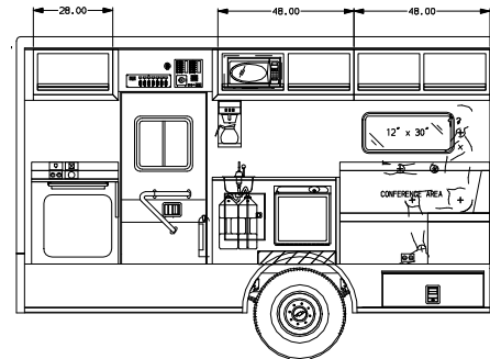
FLOORPLAN "C"
