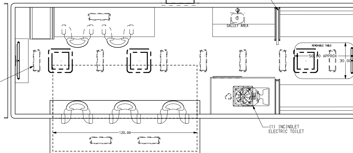
PASSENGER'S SIDE INTERIOR SECT. A-A
