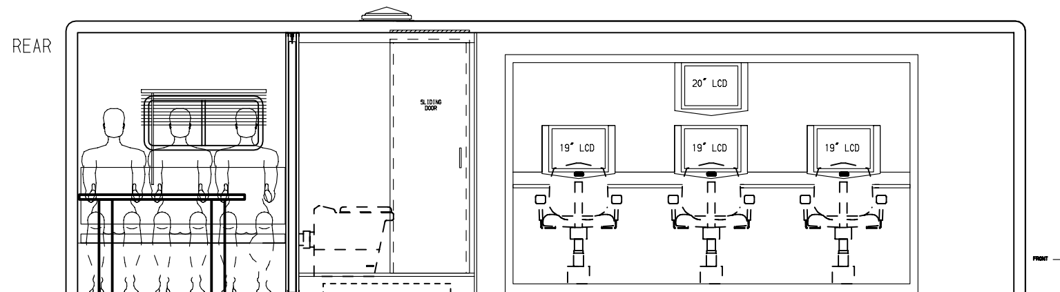
DRIVER'S SIDE INTERIOR SECT. A-A
