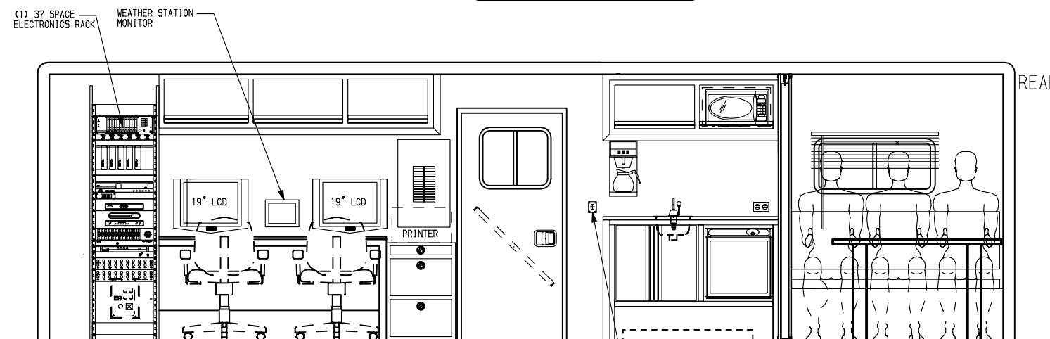
PASSENGER'S SIDE INTERIOR SECT. A-A
